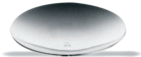
mm. 1,2 Platto concavo Ø cm. 14 Ø 5 1 / 2 " Crescent plate Ø cm. 18 Ø 7" Plateau concave Ø cm. 20 Ø 7 7 / 8 " Konkave Platte Ø cm. 22 Ø 8 5 / 8 " Plato concavo Ø cm. 24 Ø 9 1 / 2 " Ø cm. 26 Ø 10 1 / 4 " Ø cm. 28 Ø 11"
